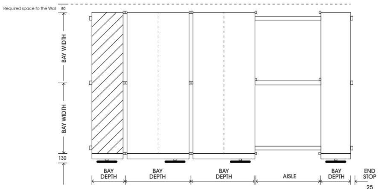
Overall Dimensions – Self Based Mechanical Assist (nominal)
