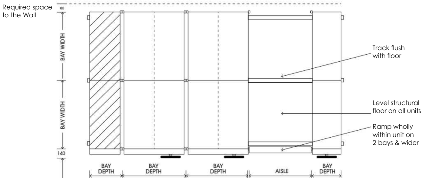
Overall Dimensions – Fixed Track Manual (nominal)
